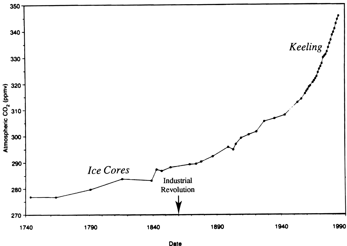
FIGURE 2. An extension of the Keeling annual means back to 1740, using measurements made on Antarctic ice cores. 2
