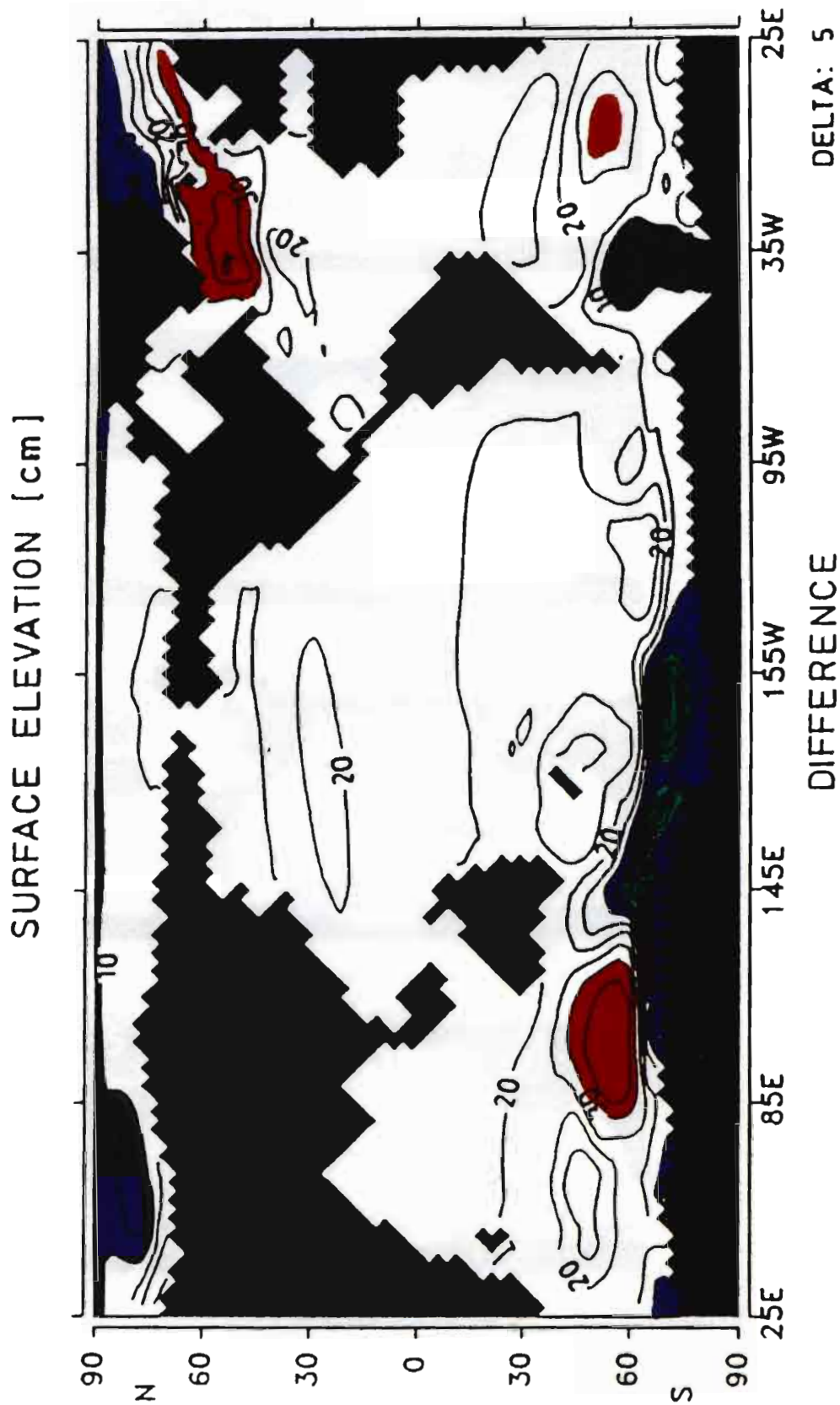
FIGURE 18. The change in sea level 50 years following CO 2 doubling. 14
