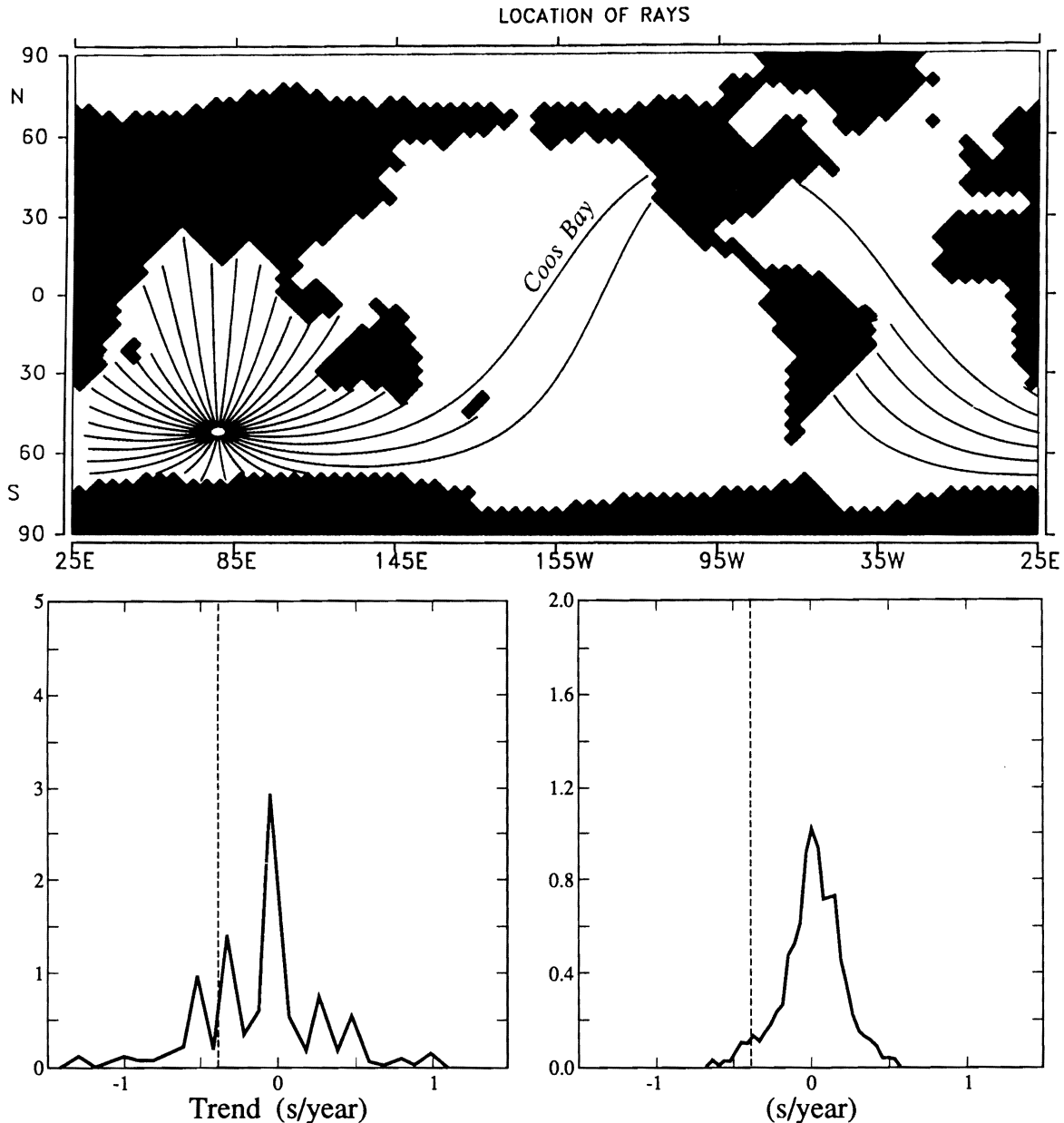
FIGURE 20. The vertical dashed line corresponds to a deterministic change in travel time by -0.4 s/year as a result of greenhouse warming. This is to be compared to the probability distribution of travel time changes (heavy line) from ambient ocean variability, based on 300 decade samples of the Hamburg model. 15 For a single path from Heard Island to Coos Bay (lower left) the signal is not significantly above the noise background, but for many paths (lower right) the greenhouse signal can be detected at about the 95% level. This result is very preliminary.
