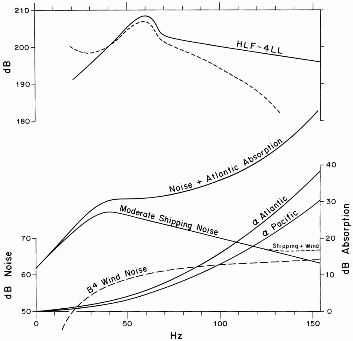
FIGURE 9. The source strength is peaked at about 60 Hz. Absorption and ambient noise limit the transmission to a 50 Hz to 70 Hz band. 9
