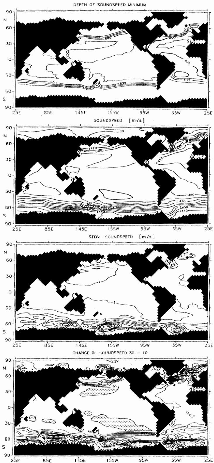
FIGURE 19. The upper two panels give the depth and sound speed of the sound channel according to the Hamburg model. 15 This compares favorably with the measured fields (figure 6). The lower two panels show the ambient variability and the greenhouse signal, respectively, of sound speed (m/s) at the sound axis.
