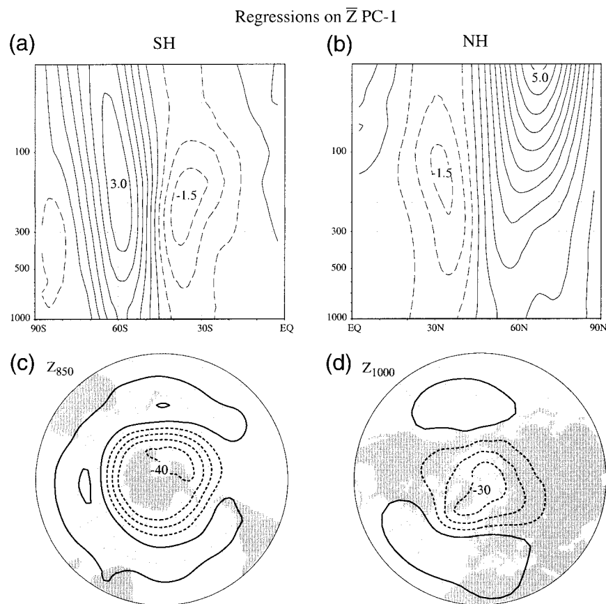
FIG. 3. As in Fig. 1, but regression maps are based on the standardized leading PC time series of the zonal-mean geopotential height field (1000–50 hPa; 20^{\circ} – 90^{\circ} ).
