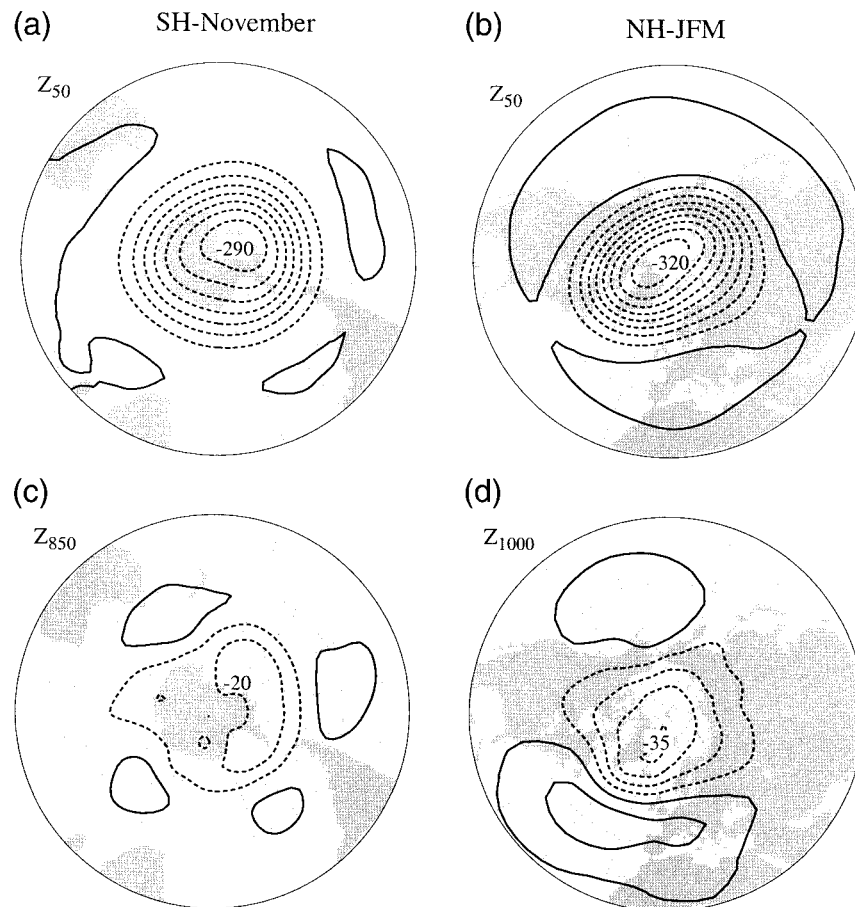
FIG. 6. (Top) Leading modal structures of the monthly mean 50-hPa height anomaly field for Nov (SH) and Jan–Mar (NH) displayed as regression maps based on their standardized PC time series. (Bottom) 1000- (NH) and 850-hPa (SH) height fields regressed onto the leading PC time series of the 50-hPa height modes depicted above. Contour intervals as in Fig. 1 for 1000- and 850-hPa height and 40 m (–60, –20, 20, . . .) for 50-hPa height.
